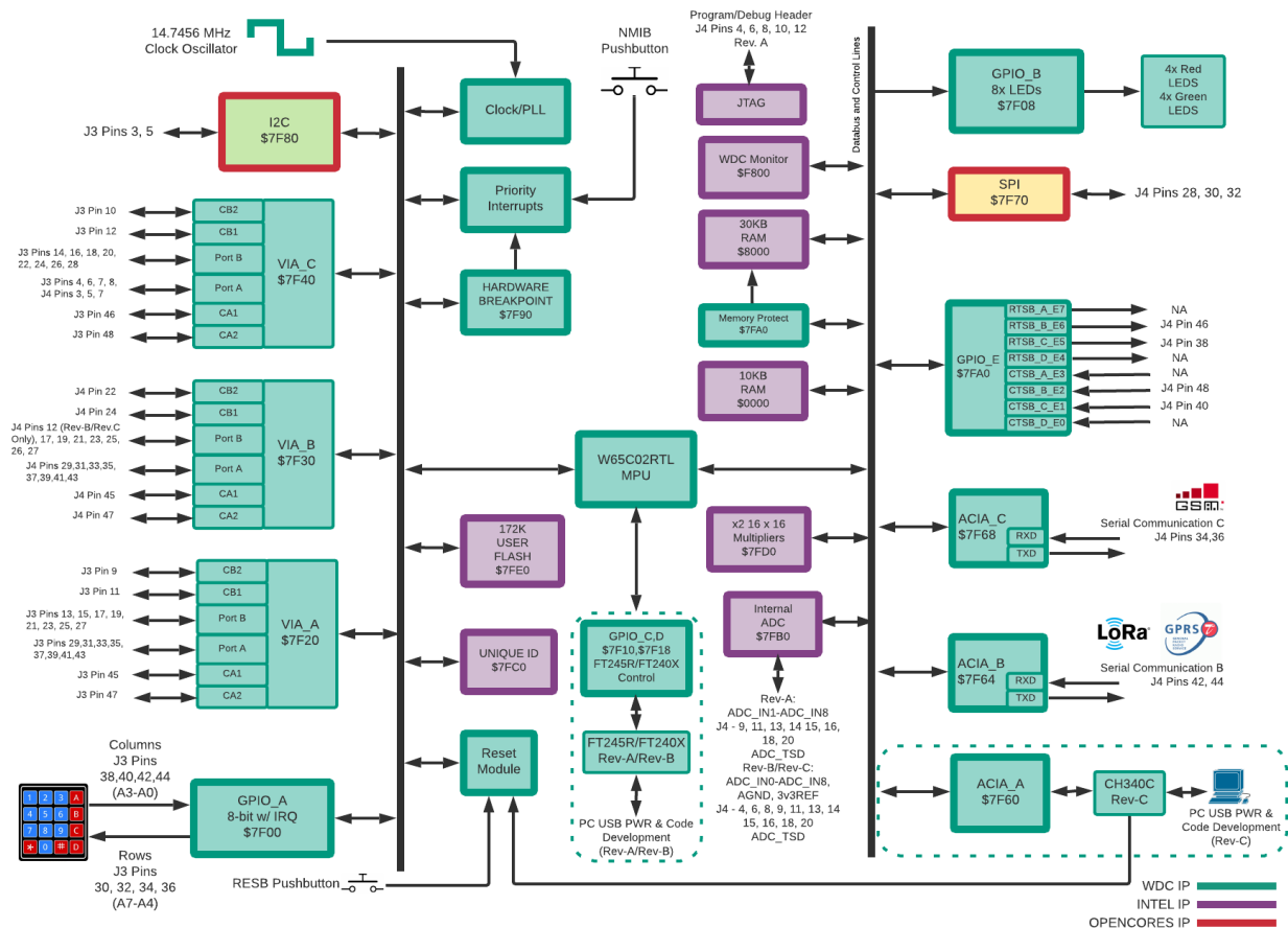
W65C165i1M08SA Functional Block Diagram (MyMENSCH Rev A/B/C)
